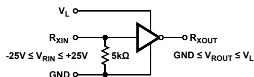
Figure 6. Receiver Connections
