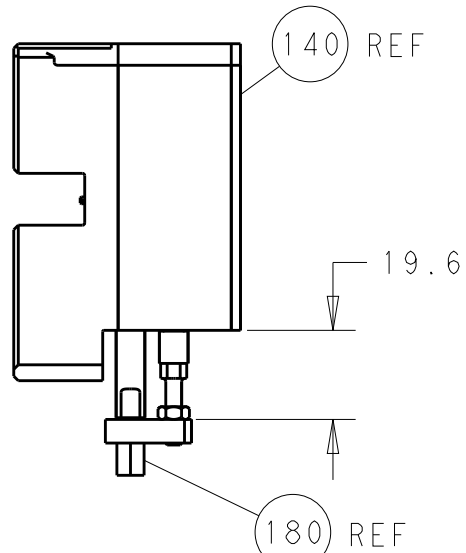
HOLDDOWN SET-UP
