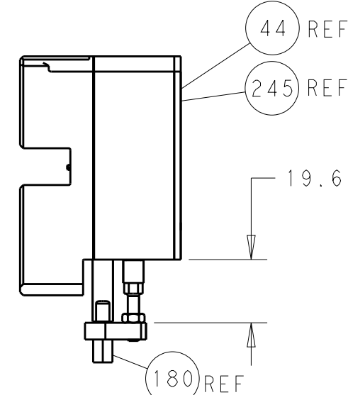
HOLDDOWN SET-UP
