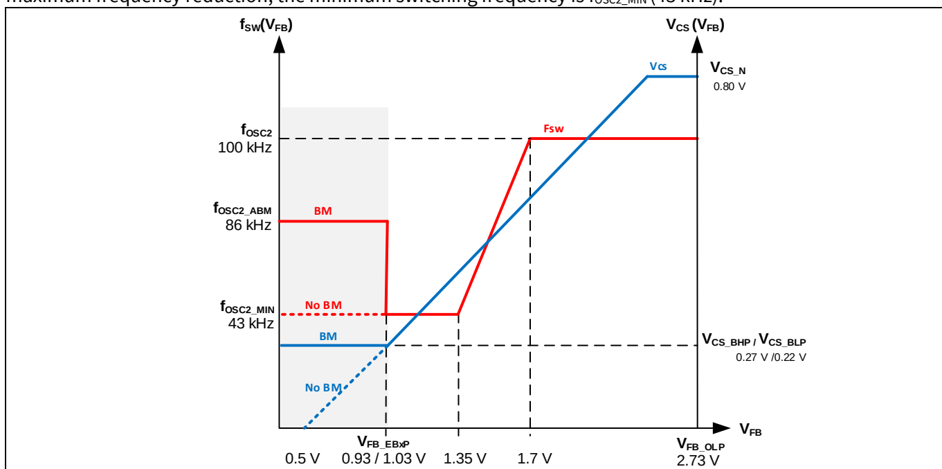
Figure 2 Frequency-reduction curve
