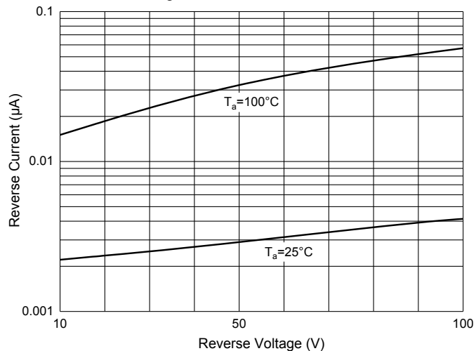
Fig. 2 - Reverse Characteristics
