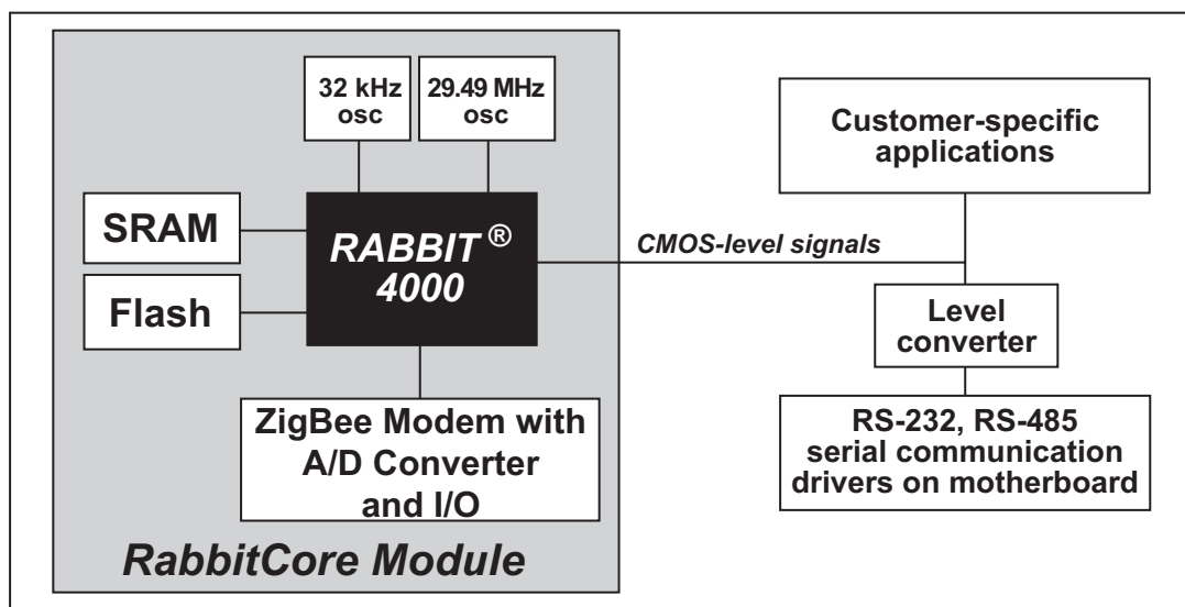
Figure 6. RCM4510W Subsystems
