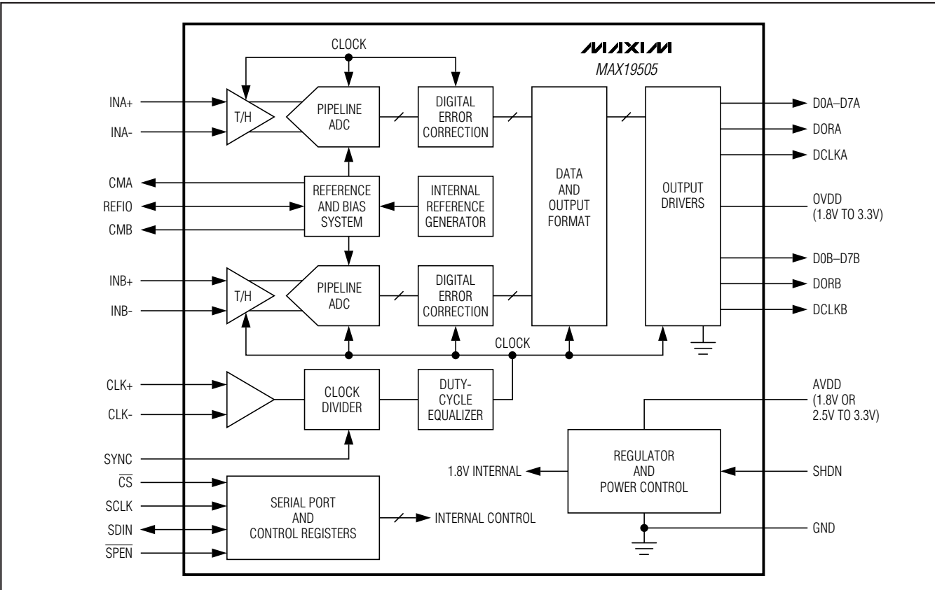
Figure 2. Functional Diagram
