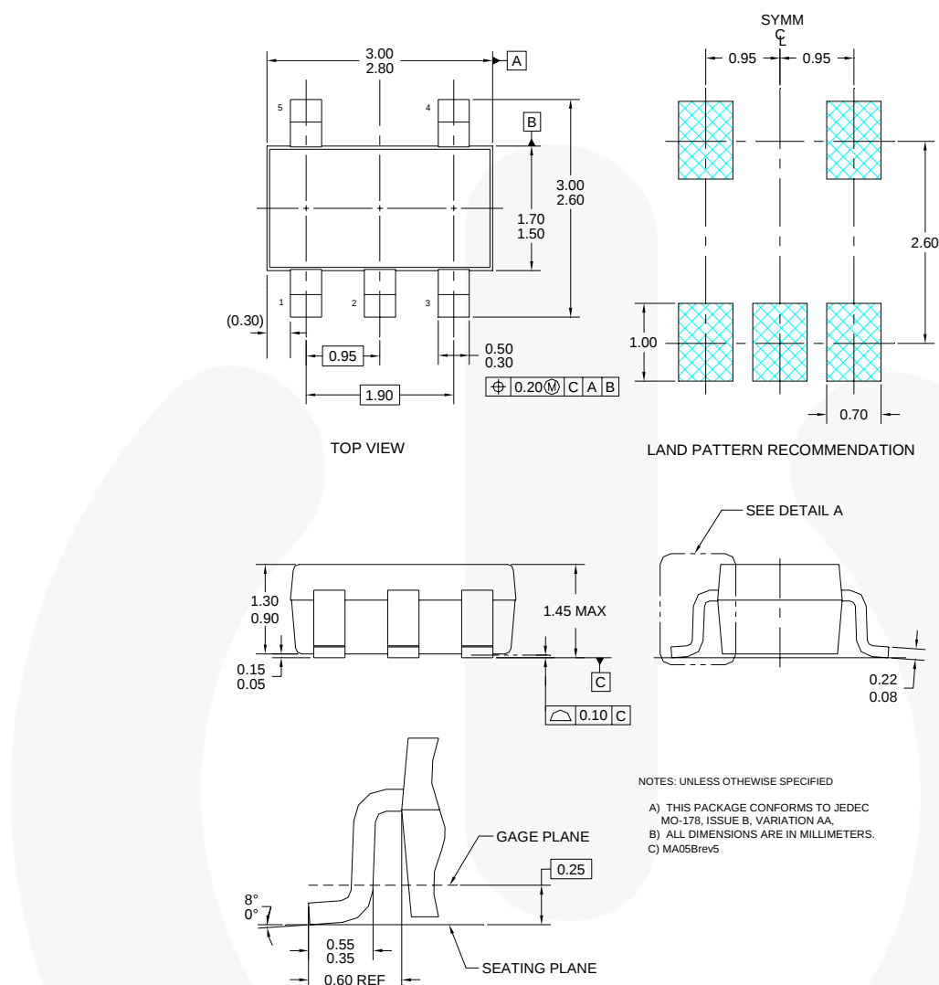
Figure 7. 5-Lead SOT23, JEDEC MO-178 1.6mm
