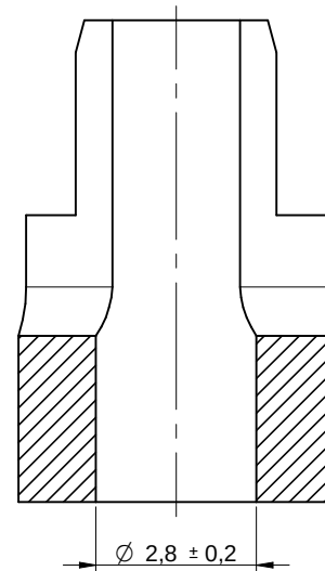
sectional drawing A-A
