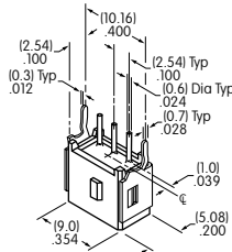
B1 Straight with Inline Bracket Single Pole only
