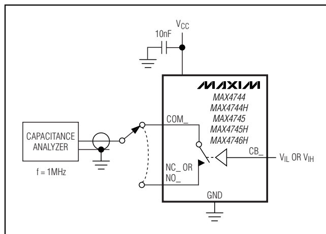
Figure 6. Channel Off-/On-Capacitance
