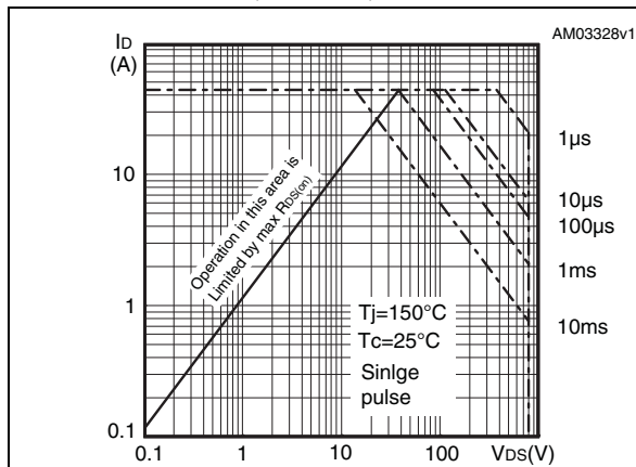
Figure 2. Safe operating area for D 2 PAK, I 2 PAK, TO-220, TO-247
