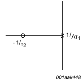
c. Pole zero diagram
