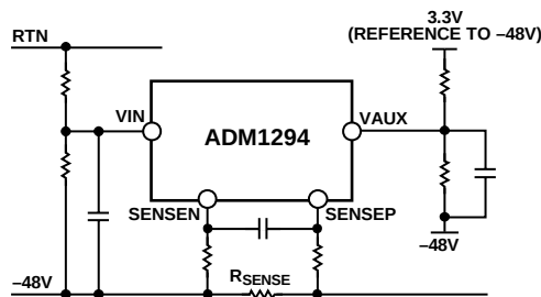
Figure 29. Power Monitor Input Filters for the ADM1294
