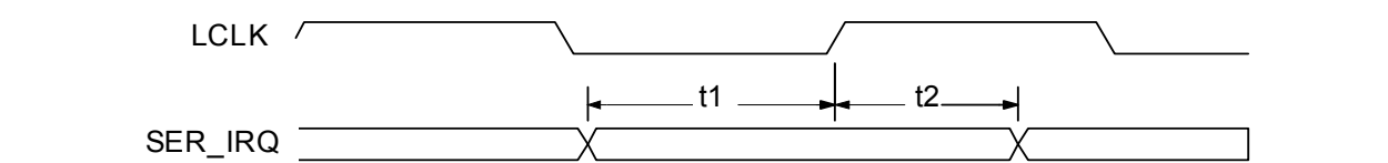
FIGURE 43-20: SETUP AND HOLD TIME
