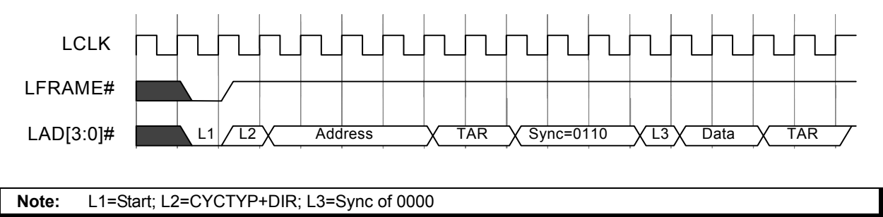
FIGURE 43-19: I/O READ
