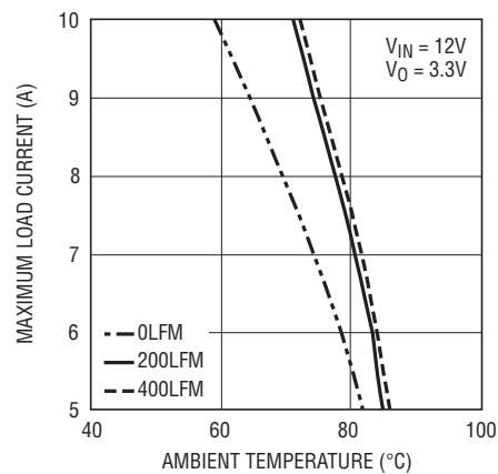
Figure 15. BGA Heatsink
