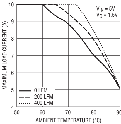
Figure 9. No Heatsink
