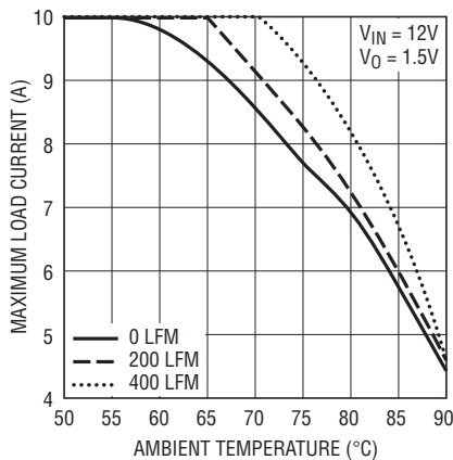
Figure 11. No Heatsink
