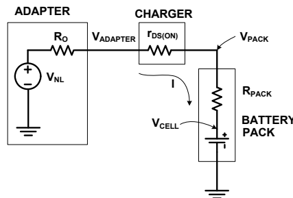
FIGURE 27B. THE EQUIVALENT CIRCUIT IN THE RESISTANCE-LIMIT REGION
