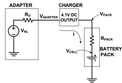
FIGURE 27C. THE EQUIVALENT CIRCUIT WHEN THE PACK VOLTAGE REACHES THE FINAL CHARGE VOLTAGE
