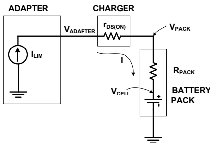
FIGURE 27A. THE EQUIVALENT CIRCUIT IN THE CONSTANT CURRENT REGION
