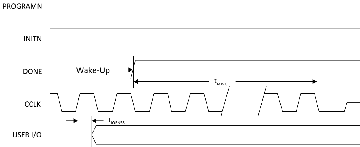
Figure 3.21. Wake-Up Timing
