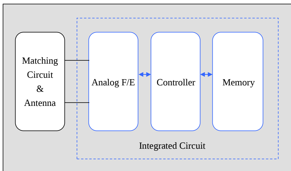
Fig.1 MAGICSTRAP®Block Diagram
