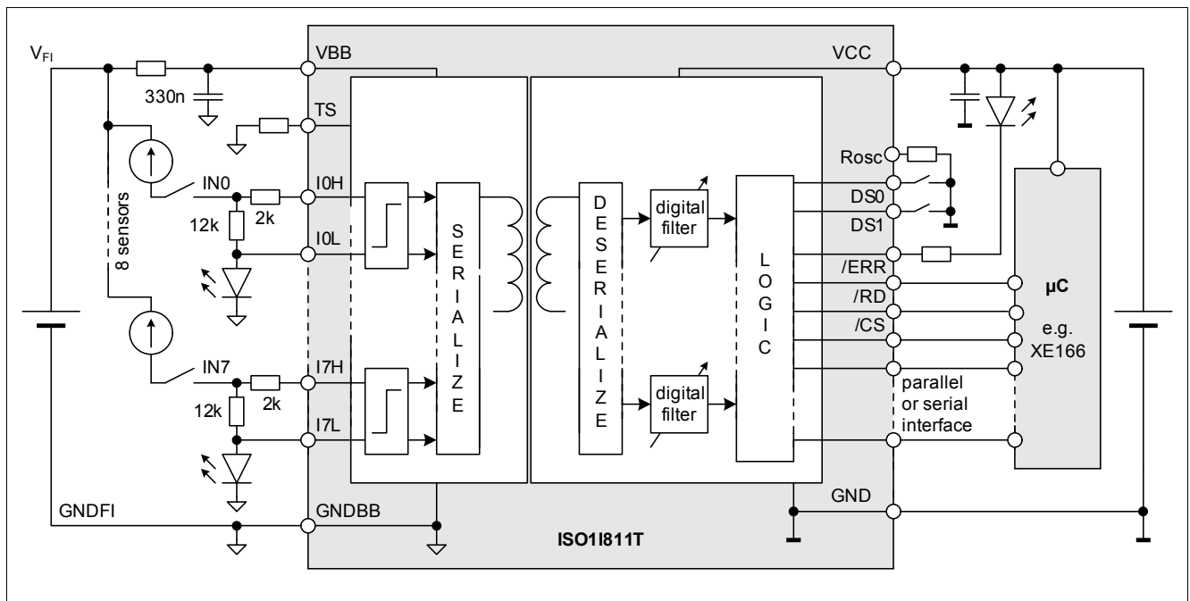
Figure 1 Typical Application
