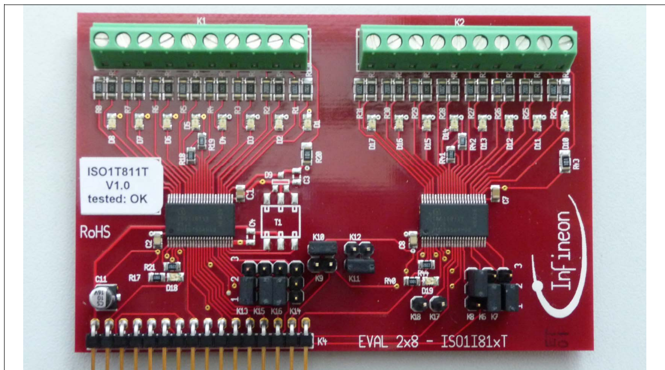
Figure 2 EVAL 2x8-ISO1I811T
