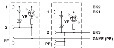
Contact assignment of the double-valve connector
