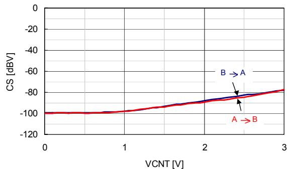
Channel Separation vs. EVR Control Voltage V+=3.5V, V_{in}=-50dBV, f=1kHz, T_a=25^{\circ}C, A\text{-Weighted}
