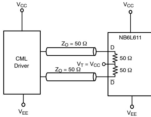
Figure 12. Standard 50 \Omega Load CML Interface
