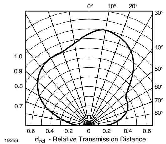
Fig. 13 - Vertical Directivity
