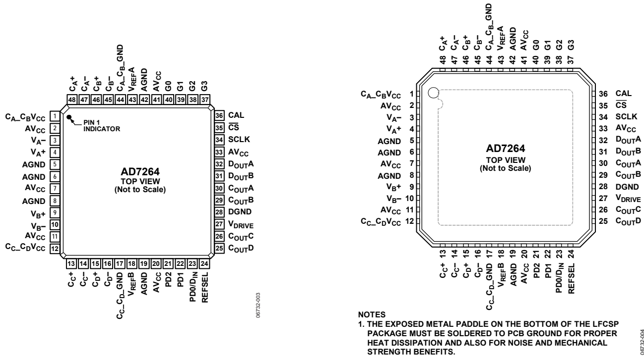
Figure 3. 48-Lead LQFP Pin Configuration
