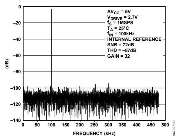
Figure 10. Typical FFT at Gain of 32
