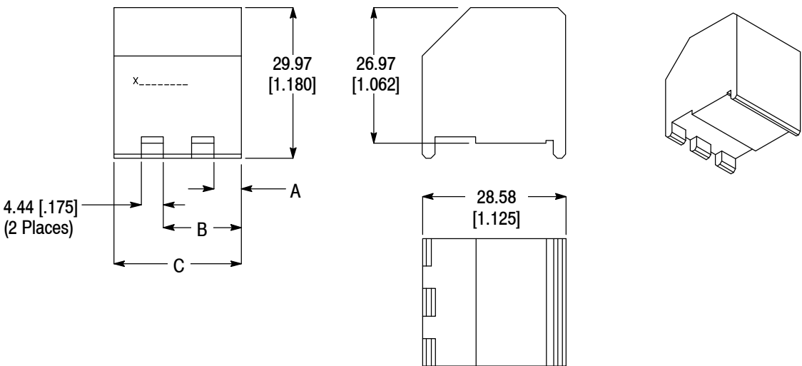
Seating Tool 91376- [ ] (3-Pair Connector)
