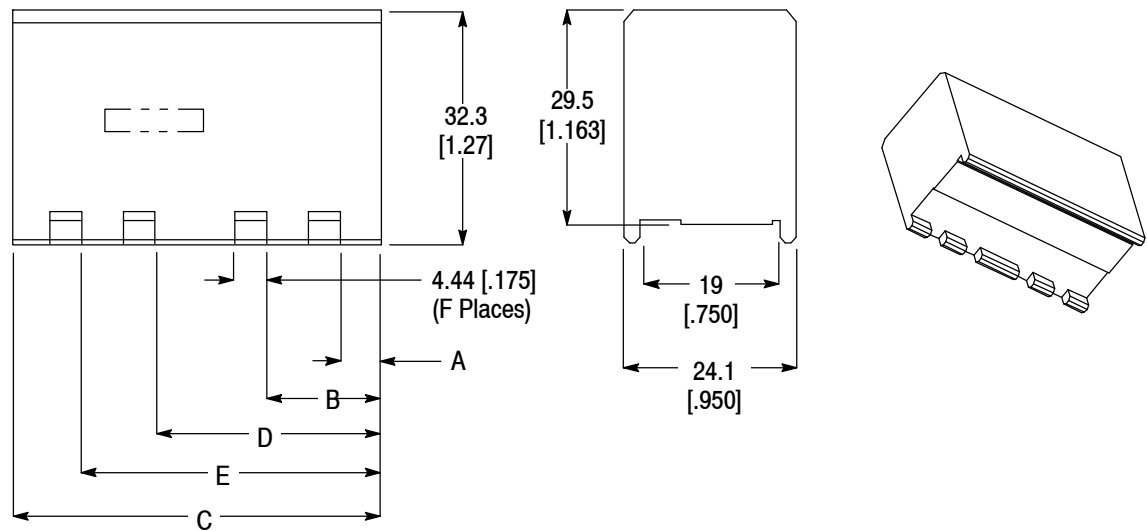
Seating Tool 91350- [ ] (2-Pair Connector)
