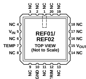
Figure 3. 20-Terminal LCC (RC-Suffix; 883 Parts Only)
