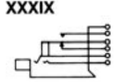
Double open circuit. Isolated switching—“break” before “make” circuit.
