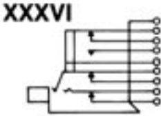
Double closed circuit. Isolated switching—One “make” and one “break” circuit.
