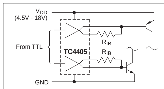
FIGURE 3-3: Driving Bipolar Transistors
