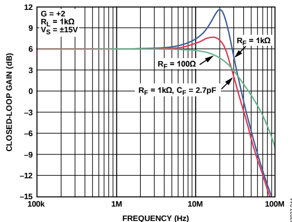
Figure 48. Small Signal Frequency Response for Various Feedback Impedances
