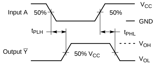
Figure 5. Switching Waveforms
