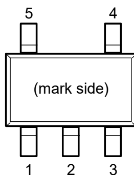
SOT-23-5 Pin Configuration
