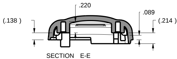
SECTION E-E
