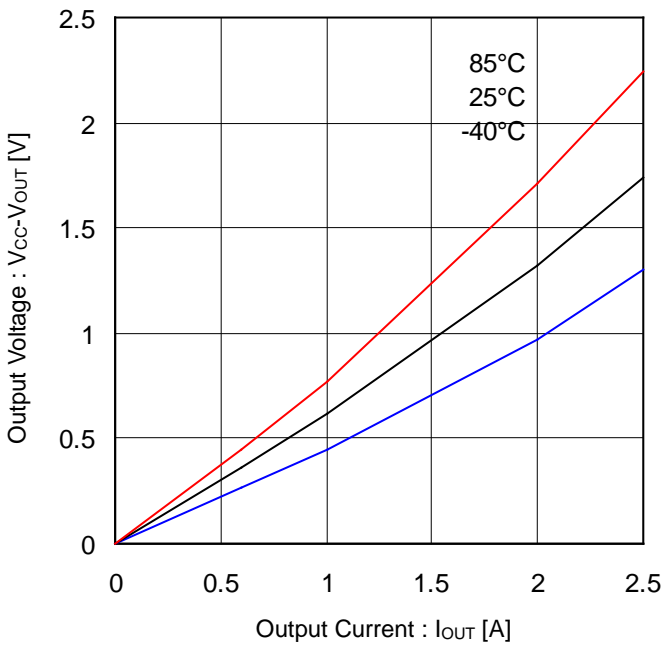
Figure 7. Output Voltage vs Output Current (Output High Voltage)
