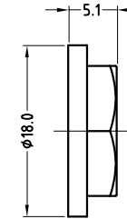
PLASTIC NUT
