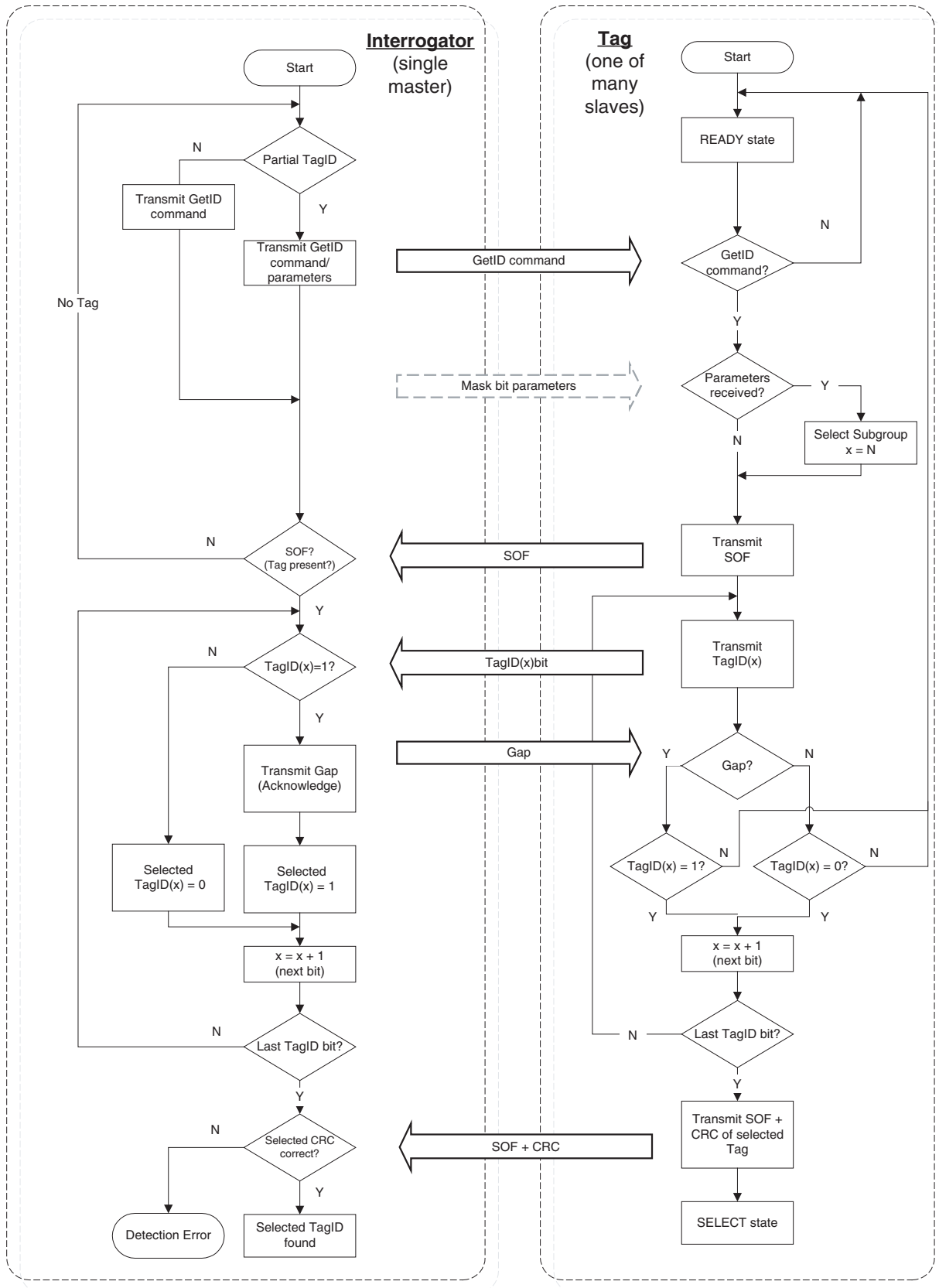
Figure 6-1. Anticollision Loop
