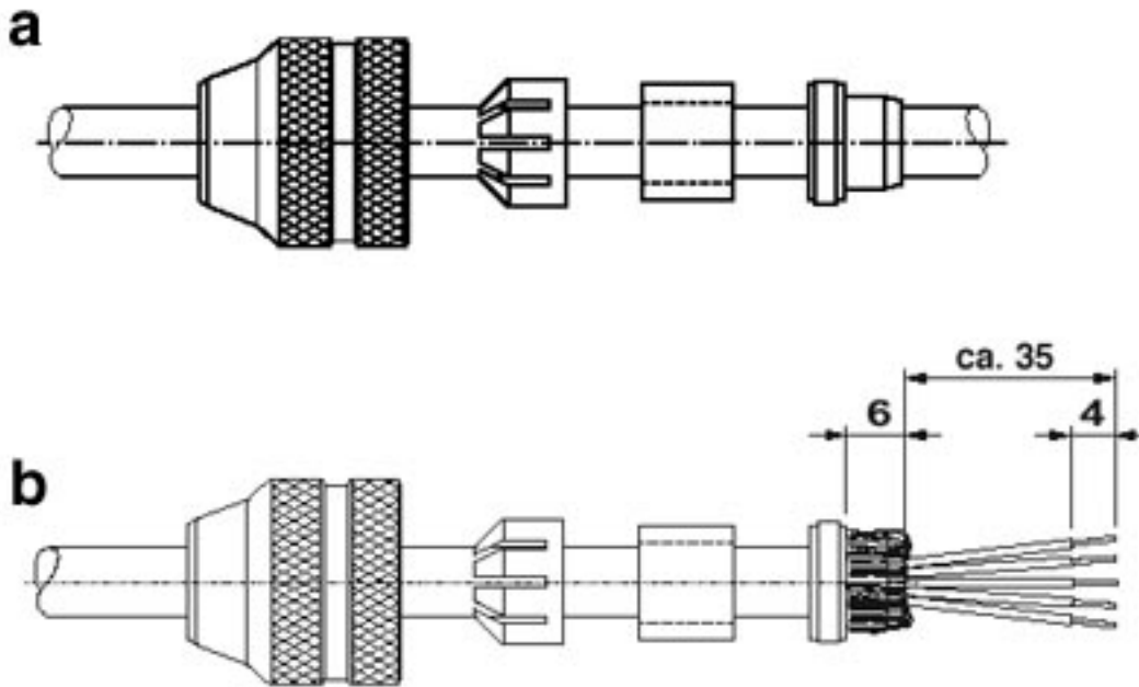
Functional drawing
