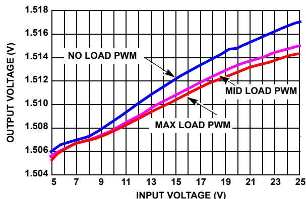
FIGURE 15. V_{OUT1} = 1.5V OUTPUT VOLTAGE REGULATION vs V_{IN} (PWM MODE)
