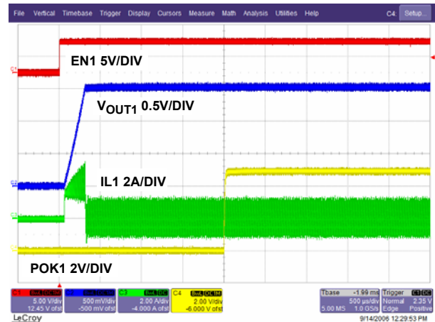
FIGURE 54. START-UP V_{OUT1} = 1.5V (NO LOAD, PWM MODE)
