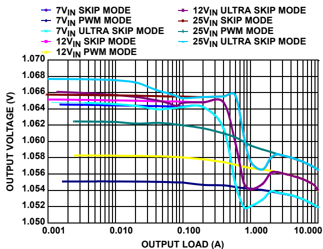
FIGURE 5. V_{OUT2} = 1.05V REGULATION vs LOAD (300kHz)
