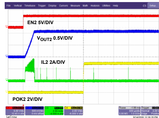
FIGURE 56. START-UP V_{OUT2} = 1.05V (NO LOAD, SKIP MODE)
