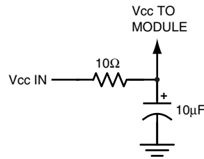
Figure 111: Supply Filter
