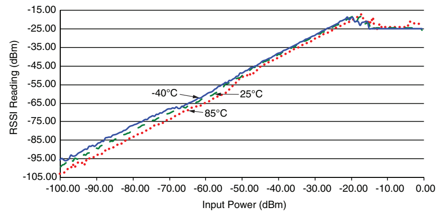
Figure 13: HumPRO™ Series Transceiver RSSI Voltage vs. Input Power - HUM-900-PRO
