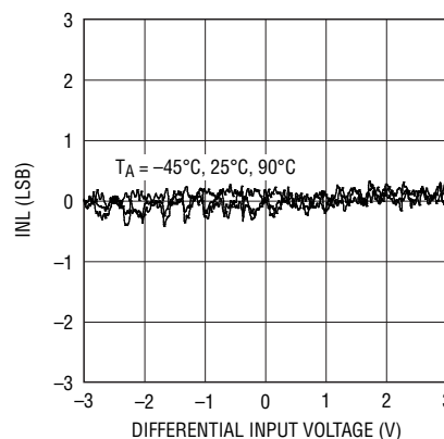
Integral Nonlinearity, V_{CC} = 3V
