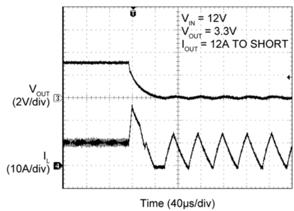
Short Circuit
