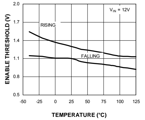
Enable Threshold vs. Temperature
