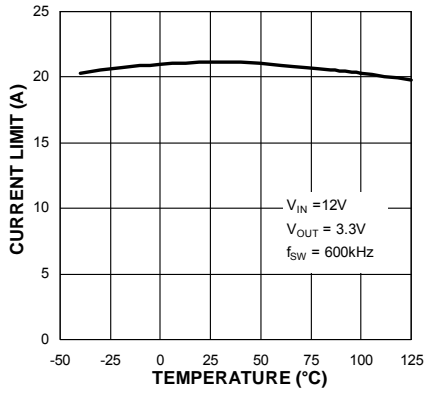
Output Peak Current Limit vs. Temperature
