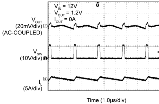
MIC2102 Switching Waveforms ( I_{OUT} = 0A )
