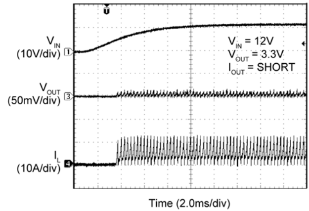
Power-Up into Short Circuit
