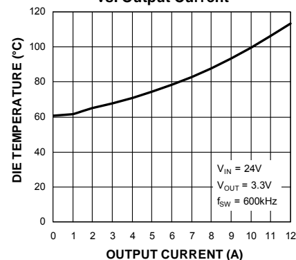
Die Temperature* ( V_{IN} = 24V ) vs. Output Current
