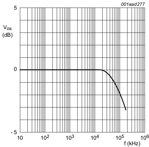
Fig 19. Frequency response
