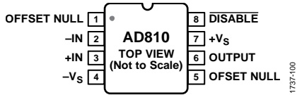
Figure 4. 8-Lead CERDIP Pin Configuration
