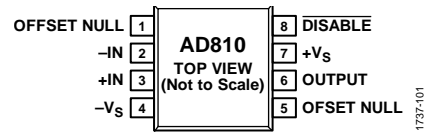
Figure 5. 8-Lead SOIC Pin Configuration
