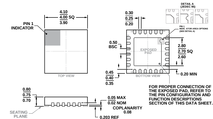
Figure 23. 24-Lead Lead Frame Chip Scale Package [LFCSP] 4 mm x 4 mm Body and 0.75 mm Package Height (CP-24-23)
