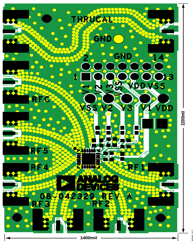
Figure 18. Evaluation Board Layout Top View
