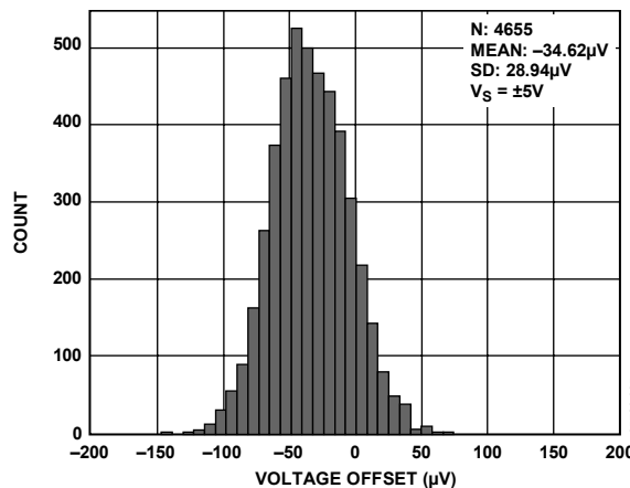
Figure 39. Input Offset Voltage Distribution ( V_S = \pm 5V )
