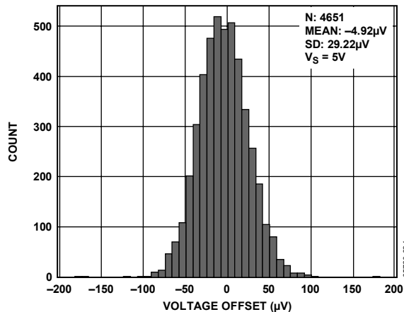
Figure 38. Input Offset Voltage Distribution ( V_S = 5V )
