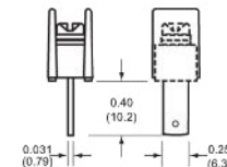
09 0.250" QC short
