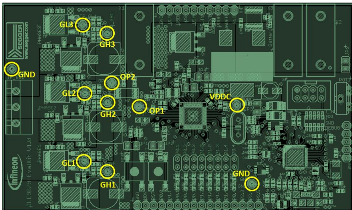
Figure 3: Test Points
