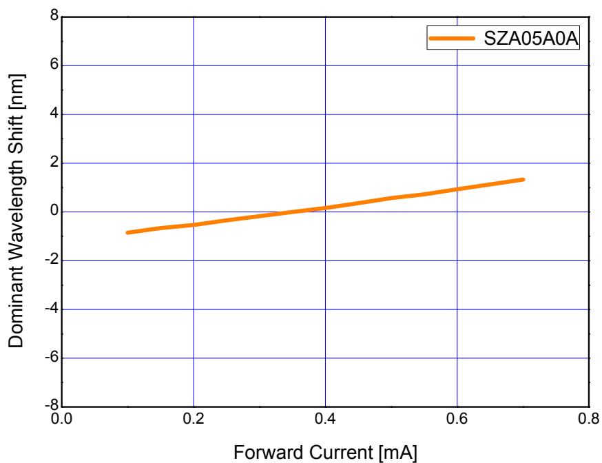
Forward Current vs Wavelength Shift, Ta=25℃
